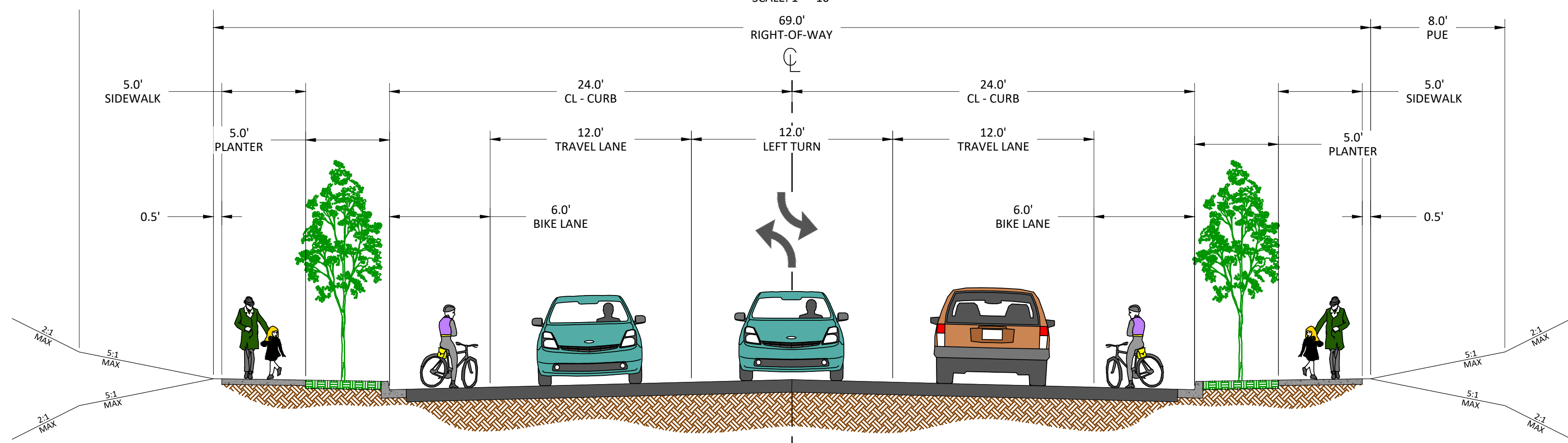
COLLECTOR ROAD (SE TROGE RD / SE CROSSROADS AVE)
