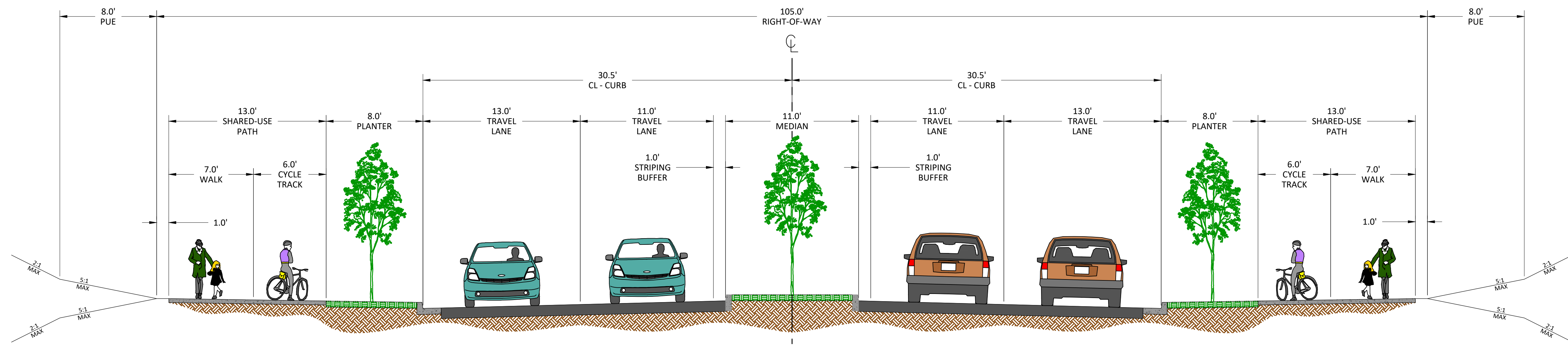
5-LANE SECTION WITH MEDIAN
