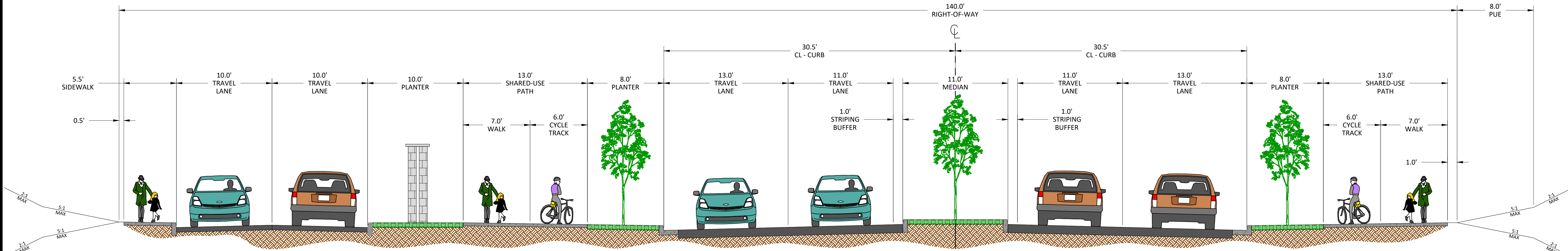
5-LANE SECTION WITH MEDIAN & FRONTAGE ROAD
