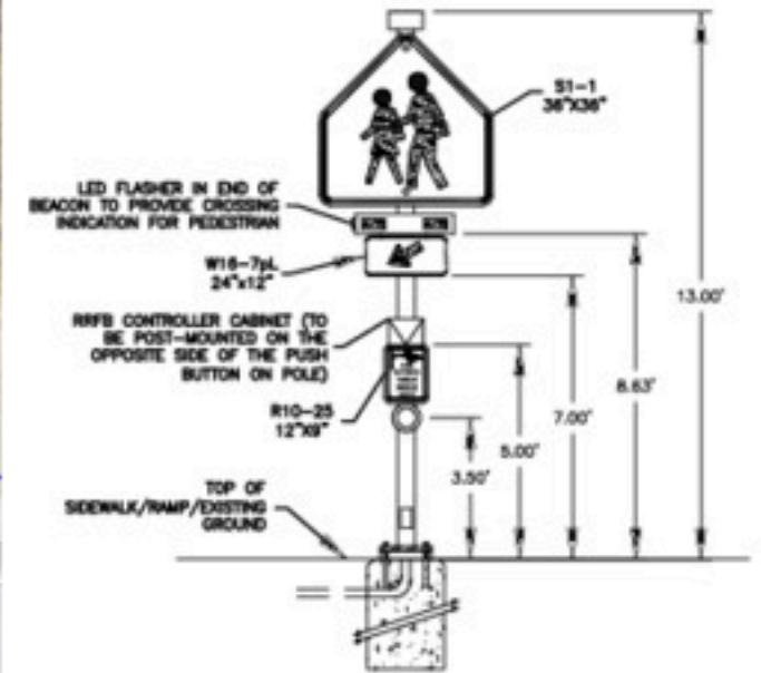
RECTANGULAR RAPID FLASHING BEACON DETAIL (NOT TO SCALE)
