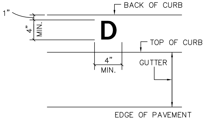
PLAN VIEW (TYPICAL)
