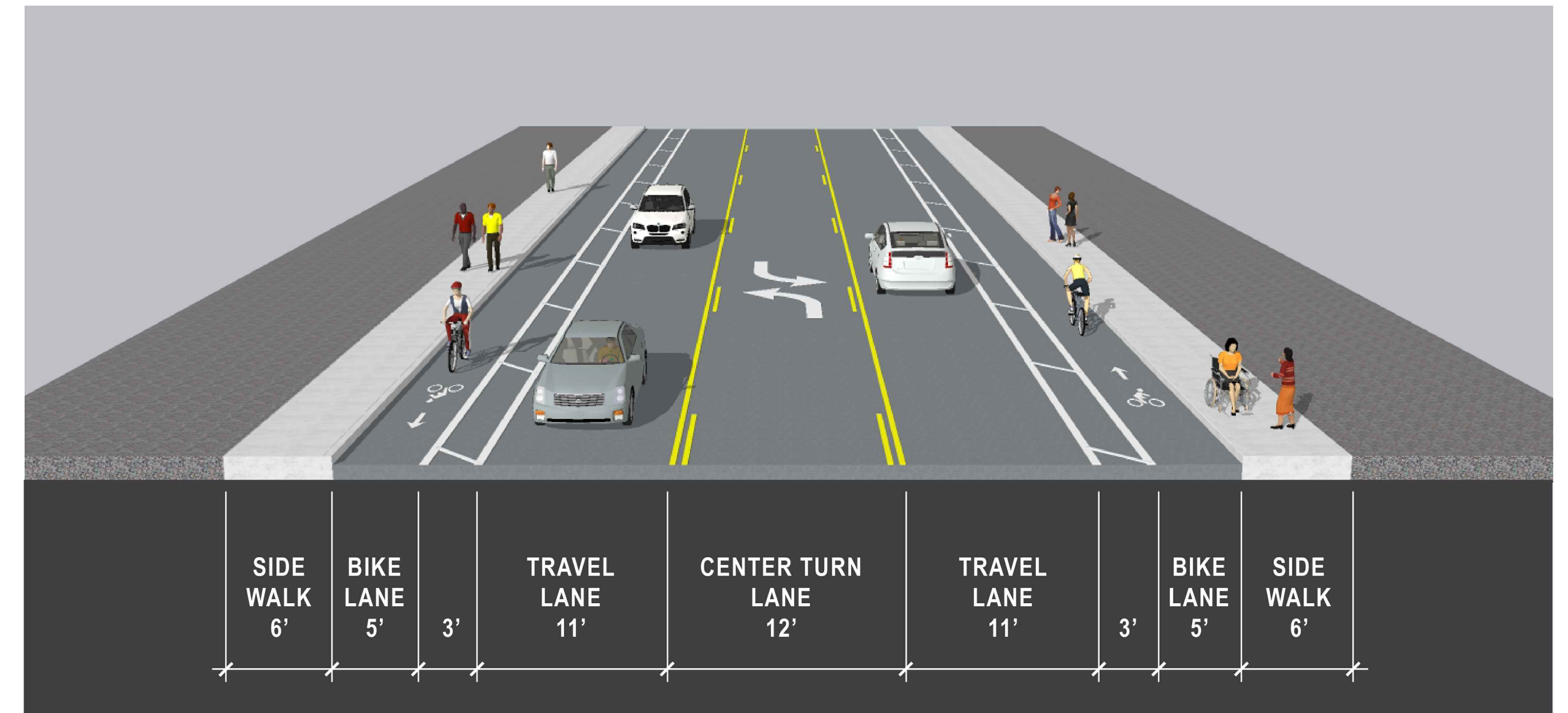
Three Travel Lanes without Landscaping
