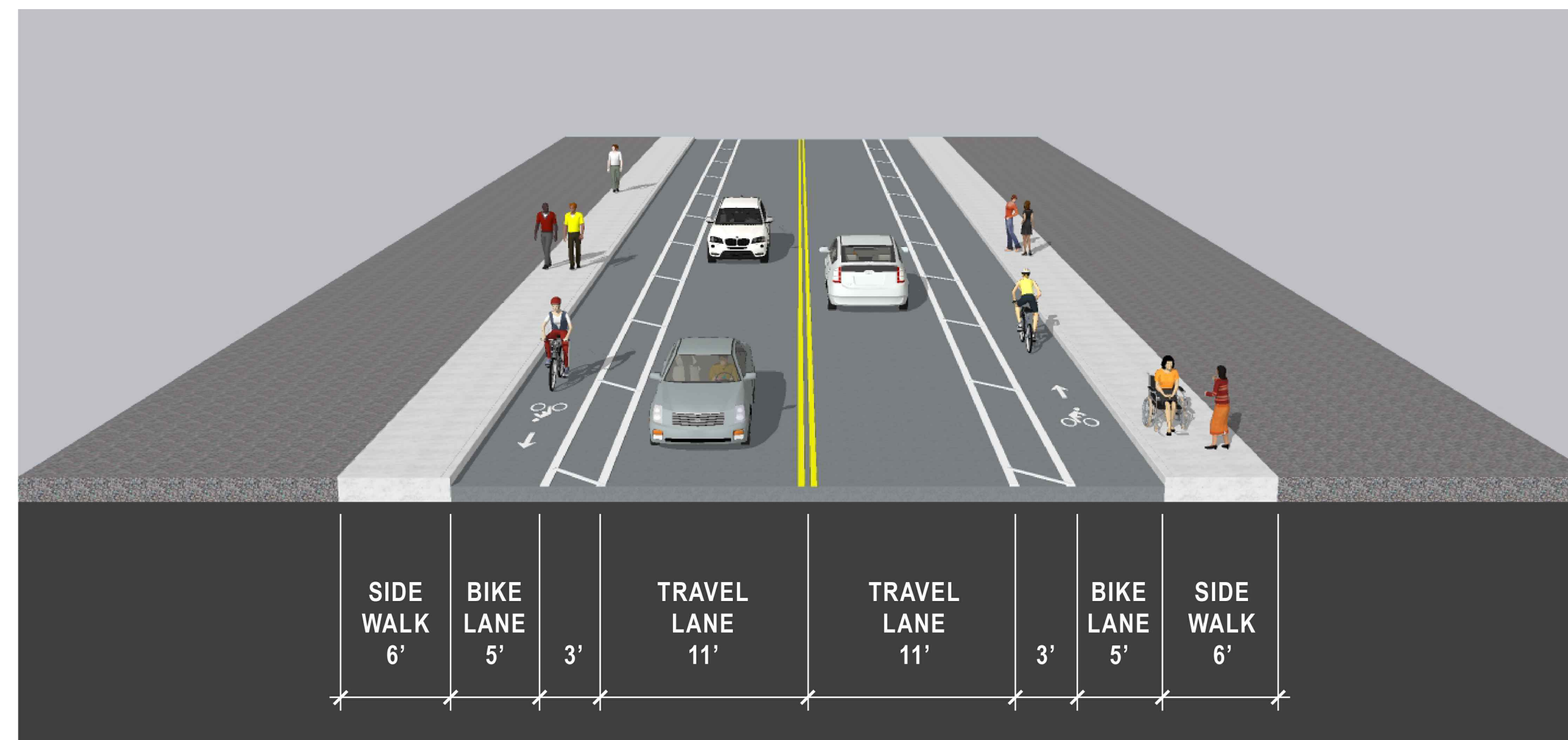
Two Travel Lanes without Landscaping
