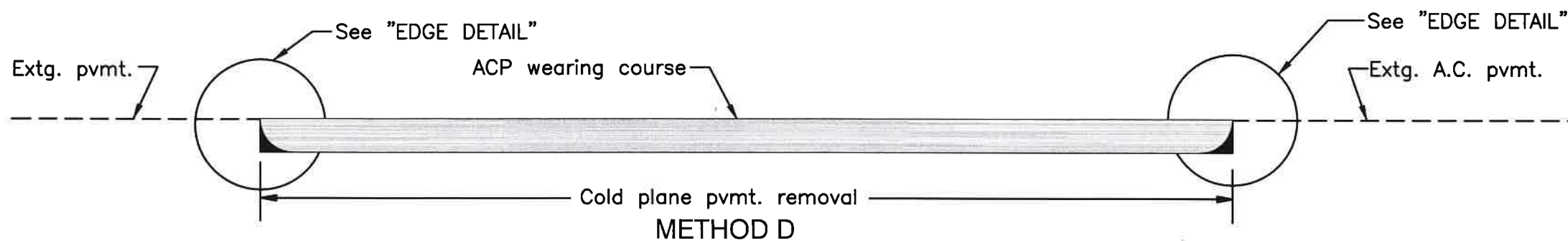
METHOD D METHOD OF MATCHING EXTG. ACP INLAY SURFACING (Inlay to extg. asphalt conc. pvmt.)
