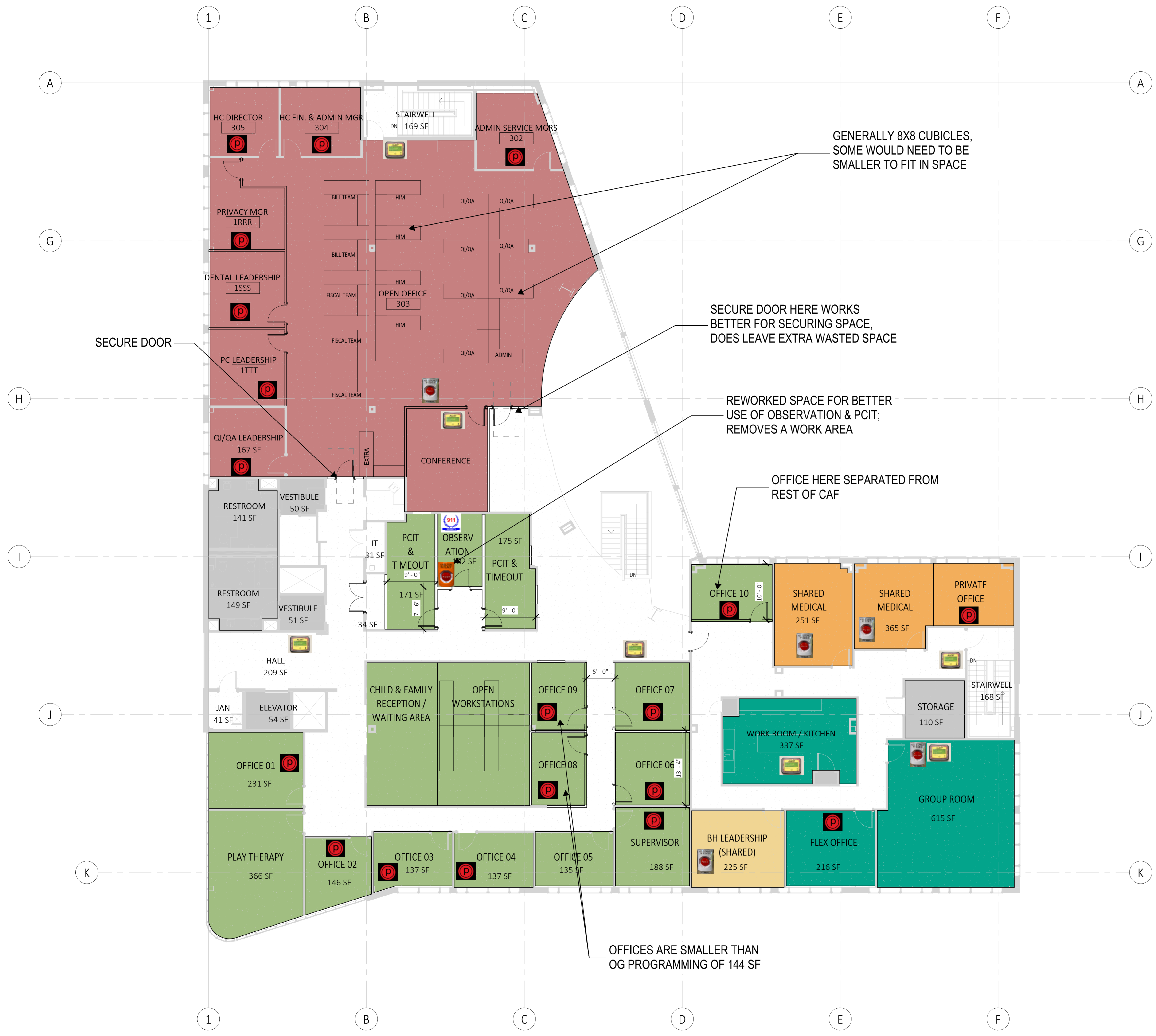
1 LEVEL 03 1/8" = 1'-0"
