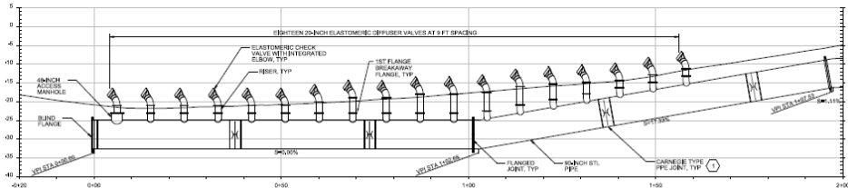
DIFFUSER PROFILE
