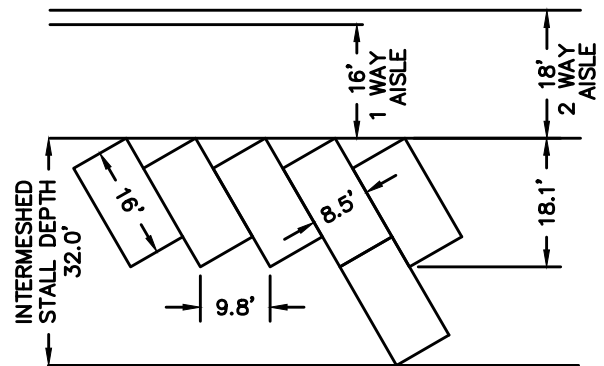
60° PARKING STANDARD STALL (8.5'x16')
