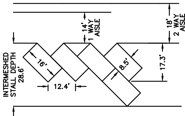
45° PARKING STANDARD STALL (8.5'x16')
