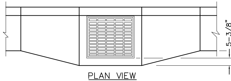
CURB AND GUTTER TRANSITION SECTION
