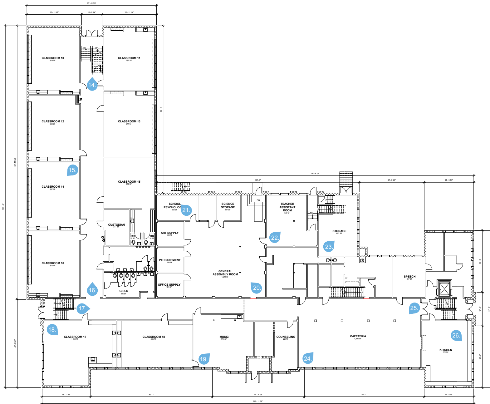
1 | LOWER LEVEL FLOOR PLAN A1.10 1/8" = 1'-0"
