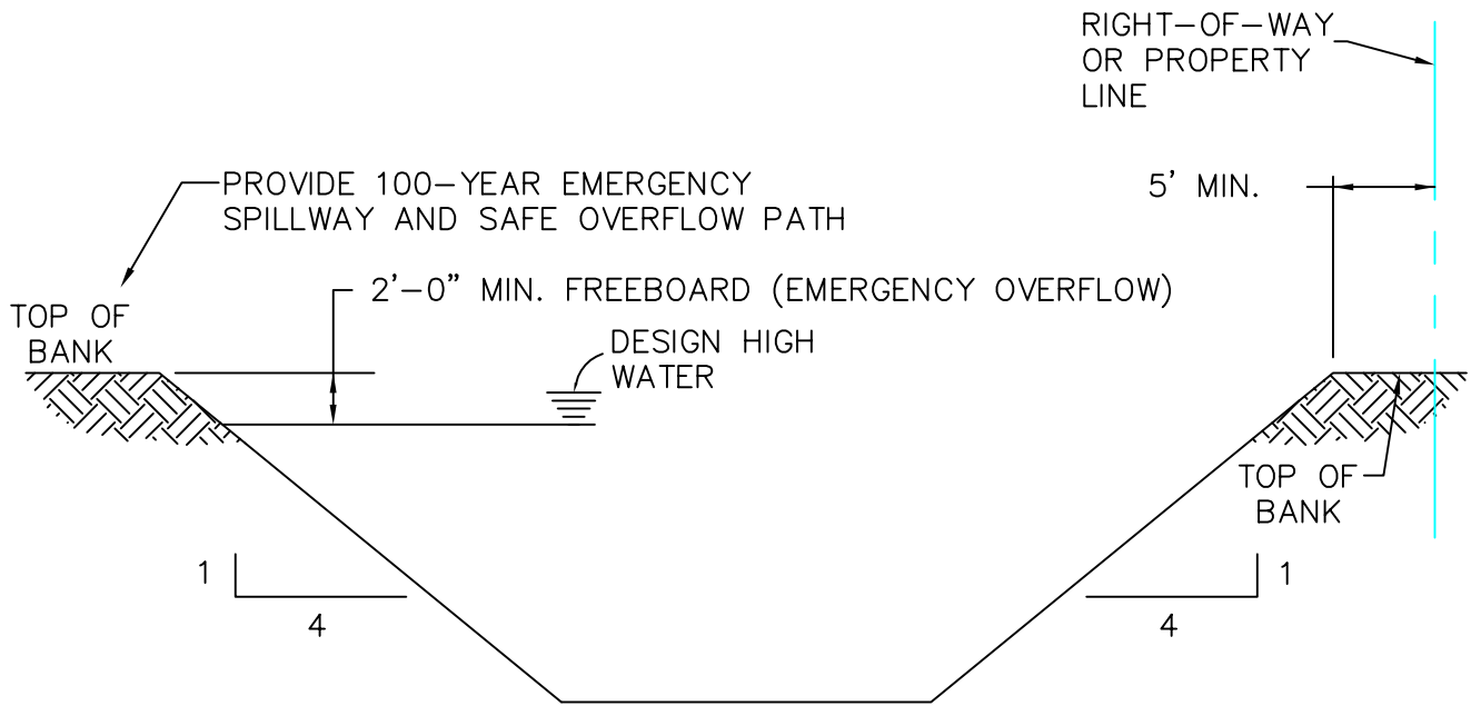
STANDARD DETENTION POND
