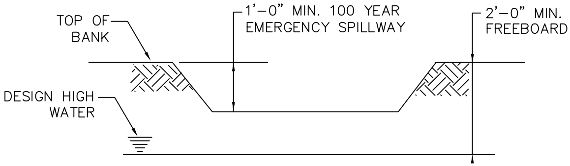
100 YEAR EMERGENCY SPILLWAY
