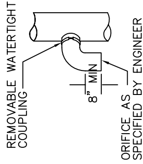
ELBOW DETAIL
