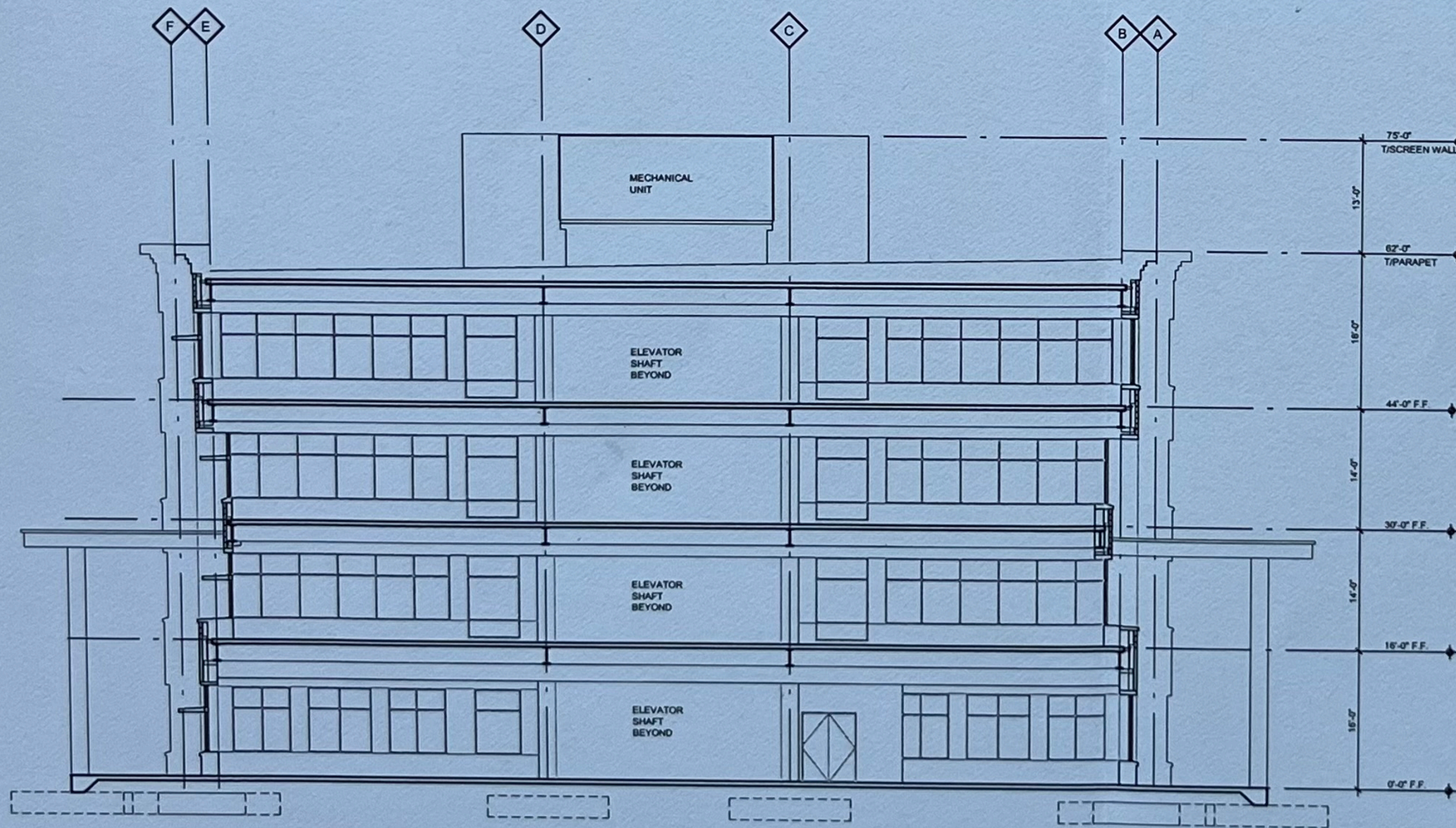
2 NORTH-SOUTH BUILDING SECTION A15 1/8"=1'-0"
