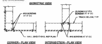
5 WALL FRAMING AT CORNERS AND INTERSECTIONS 1" = 1'-0"
