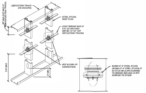
1 STEEL STUD WALL BRIDGING 1" = 1'-0"
