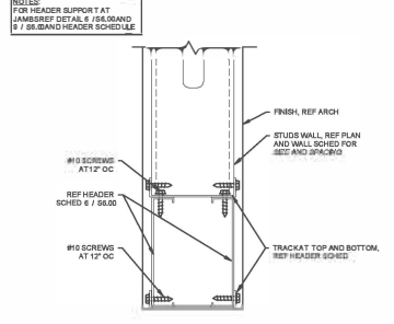
7 BOX HEADER DETAIL 1" = 1'-0"
