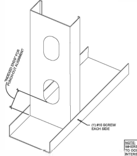
2 STUD TO TRACK ATTACHMENT 1" = 1'-0"
