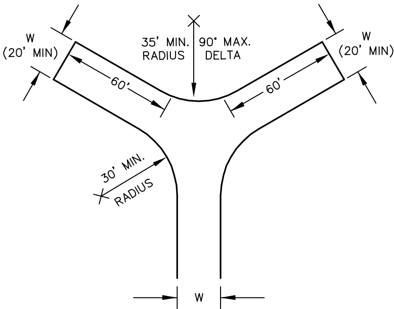
HAMMERHEAD ALTERNATIVE 1
