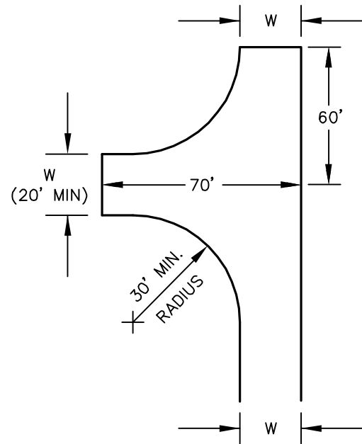
HAMMERHEAD ALTERNATIVE 2
