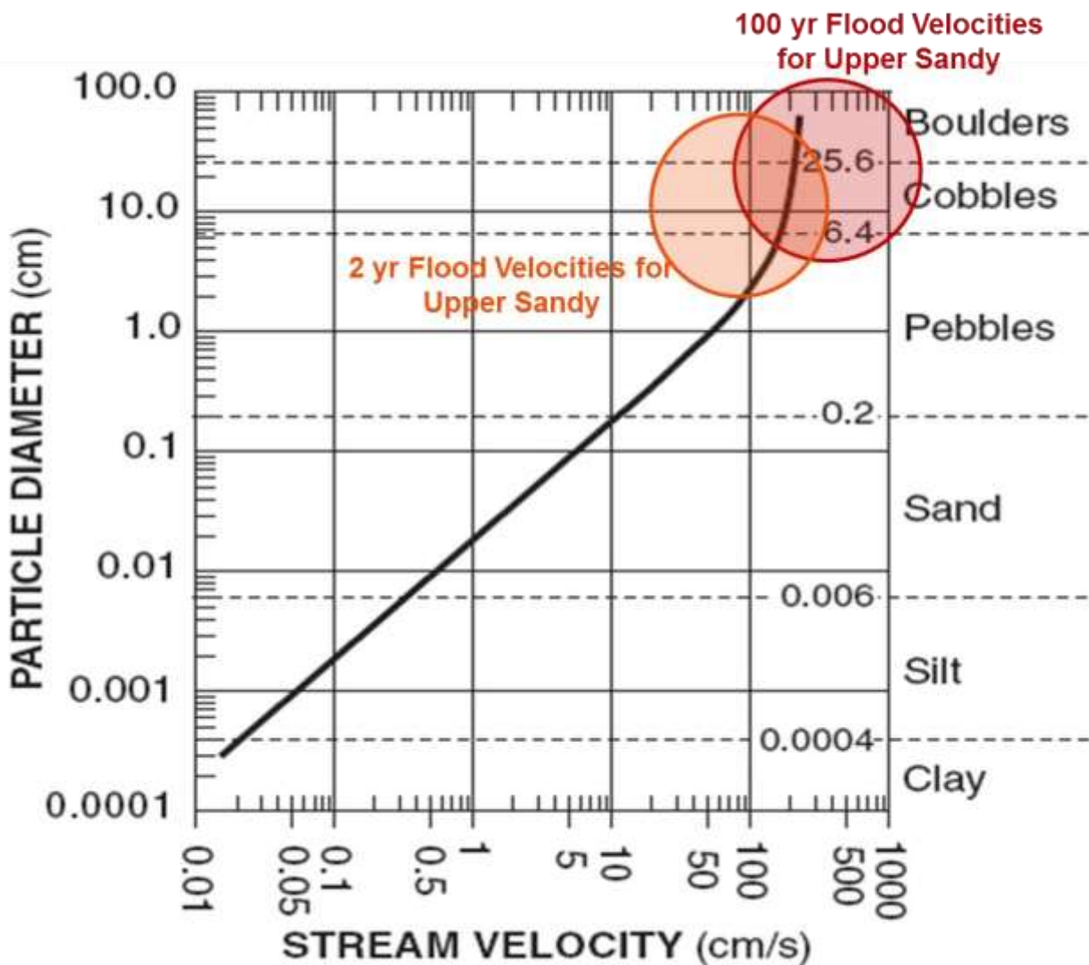
Figure 29. Relationship between flow velocity and average (D50) minimum stable particle size. This graph displays the median grain diameters stream flow can transport during the 2-year (large cobbles) and 100-year (cobble to boulders) recurrence interval storm flows. After Peter Mulroy 2012.
