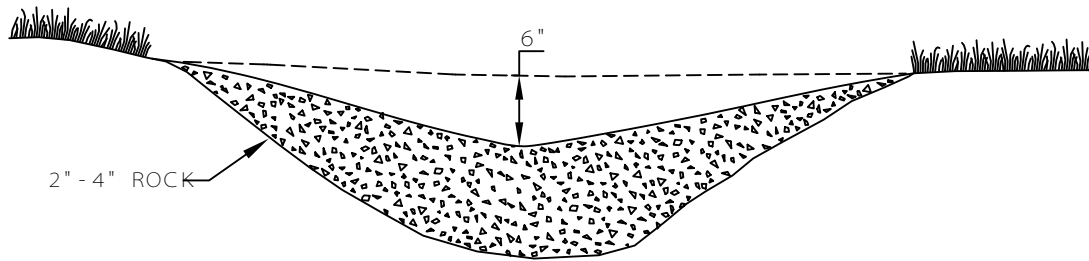
ROCK CHECK DAM
